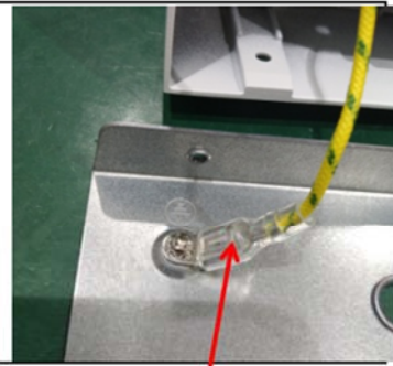
Figure 3 Remove the ground cable terminal
