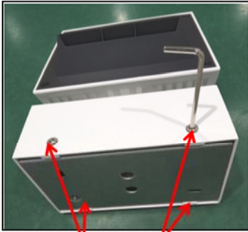
Figure 1 Remove the screws
